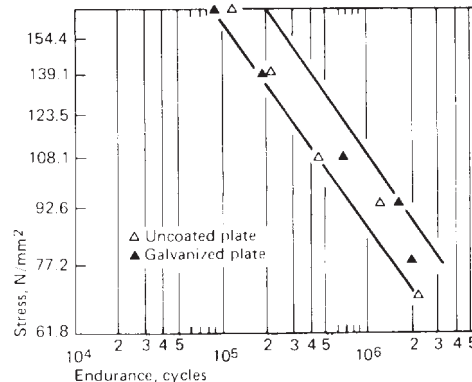
SN curves showing results of fatigue tests on cruciform joints. CO 2 short circuiting GMA welds on 13mm uncoated and galvanized Lloyds Grade A steel, AWS E60S-3 filler metal. EN Gregory, 'The mechanical properties of welds in zinc coated steel'
